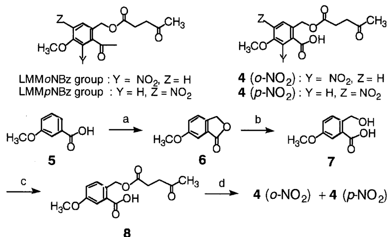
Scheme 3. Conditions: (a) HCHO, conc. HCl/1,4-dioxane, 50–55°C, 3 days, (b) 1) KOH, 85% MeOH-H 2 O, 55°C, 30 min, 2) conc. HCl, (c) levulinic anhydride, 1-methylimidazole, 1,4-dioxane, r.t., 1 h, (d) HNO 3 , H 2 SO 4 in an ice-salt bath, 20 min.
