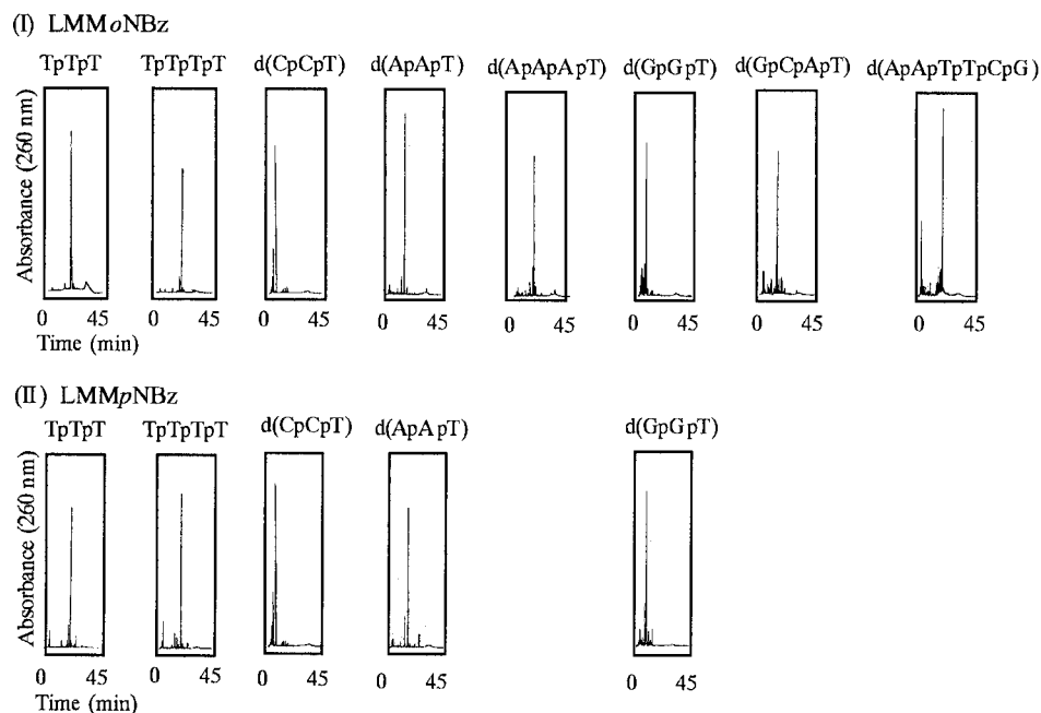
Figure 3. Reversed-phase HPLC profiles of crude products of oligodeoxyribonucleotide preparations using 3'- H -phosphonate monomers [ 10 ( o and p )] on CPGs [ 11 ( o and p )], respectively. Conditions of reversed-phase HPLC: column \mu BONDASPHERE 5 \mu C18 (3.9 mm ID \times 150 mm L); elution buffer 7.25–50% acetonitrile/0.1 M TEAA (pH 7); flow rate 1 mL/min.
