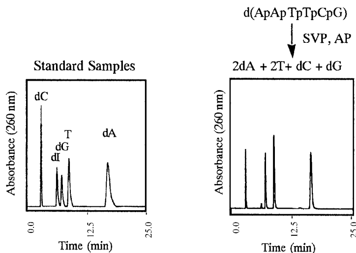
Figure 4. Reversed-phase HPLC analysis of products obtained by digestion of the completely unmasked hexamer with snake venom phosphodiesterase (SVP) and alkaline phosphatase (AP), and of standard samples. 2'-Deoxyinosine was produced from 2'-deoxyadenosine due to contamination with adenosine deaminase. Conditions of reversed-phase HPLC: column \mu BONDASPHRE 5 \mu C18 (3.9 mm ID \times 150 mm L); elution buffer 3% acetonitrile/0.06 M TEAA (pH 7); flow rate 1 mL/min.
