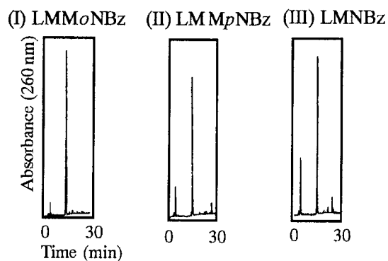
Figure 1. Reversed-phase HPLC profiles of crude products of TpT preparations using the 5'-O-DMTr-thymidine 3'-H-phosphonate 10a (DMTr) derivative on CPGs [ 11a ( o , p , and LMNBz)], respectively.
