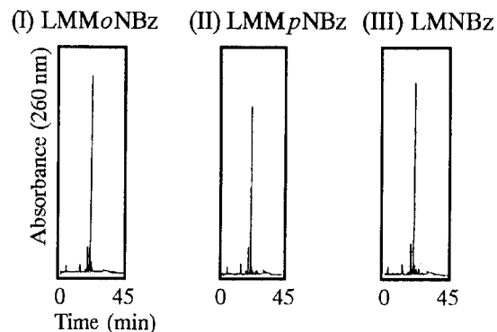
Figure 2. Reversed-phase HPLC profiles of crude products of TpTpTpT preparations using thymidine 3'-H-phosphonate derivatives [ 10a ( o , p , and LMNBz)] on CPG 11a (DMTr), respectively.
