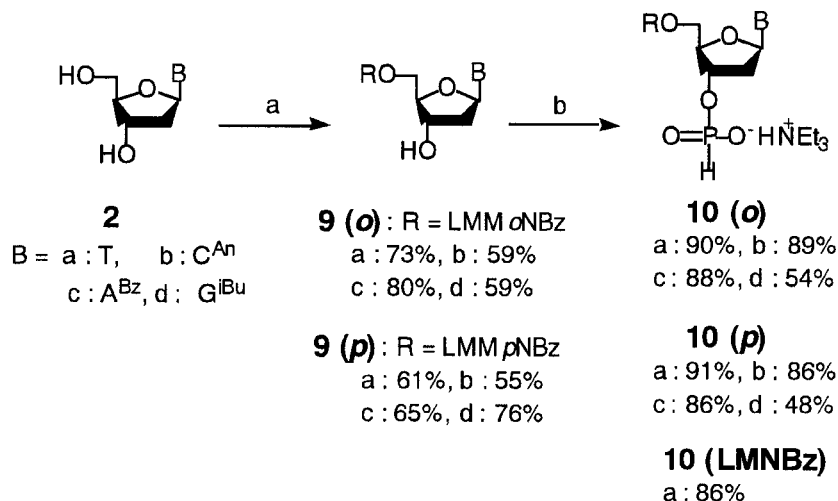
Scheme 4. Conditions: (a) 4 ( o - or p -NO 2 ), TPSCl, pyridine, r.t., 2–3 h, (b) 1) tris-(1,2,3-triazolyl)phosphine, N -methylmorpholine, CH 2 Cl 2 , 0°C, 30 min, 2) 1 M TEAB aq.
